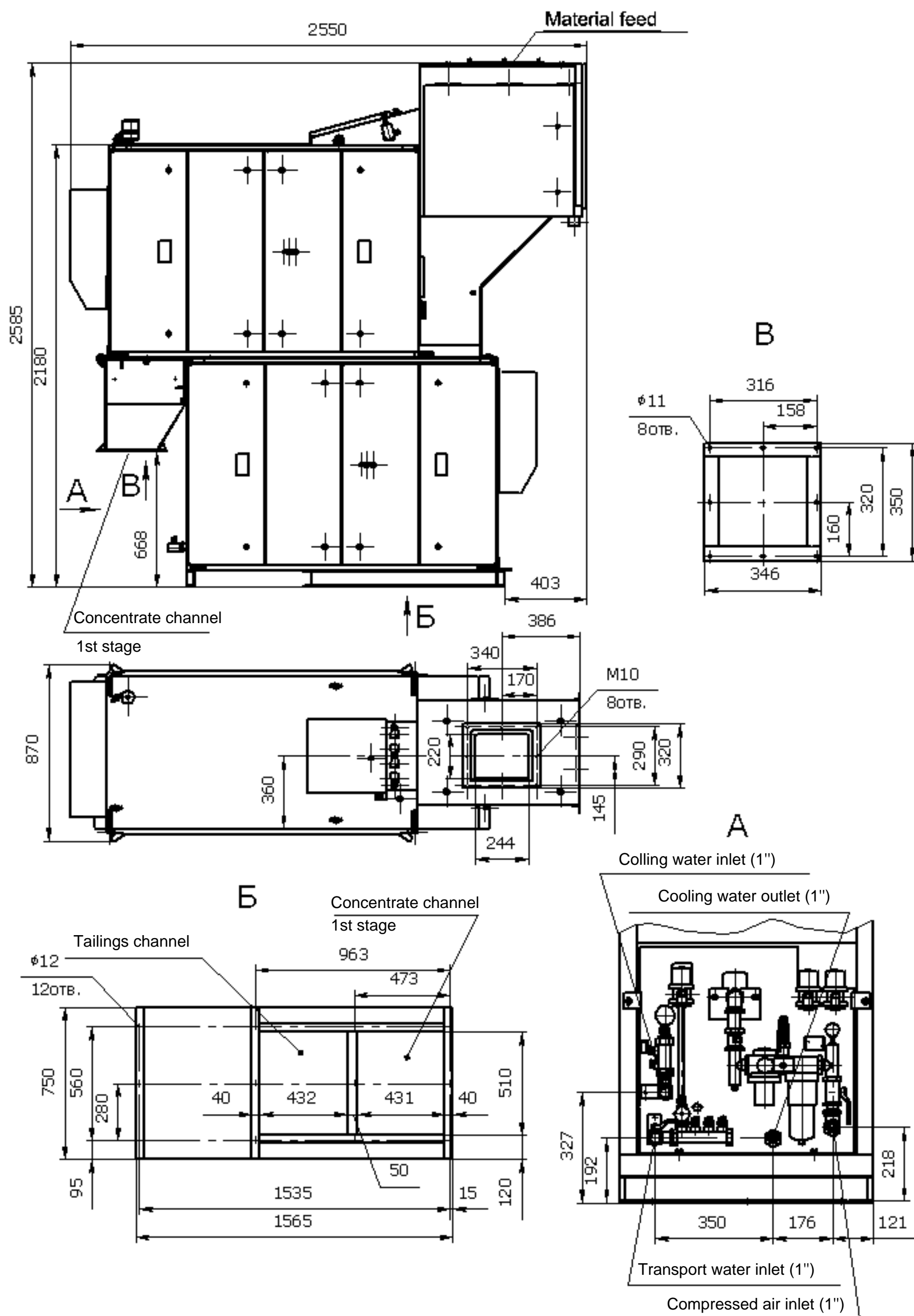
Sorting machine LS-50-05 (OKDS)
