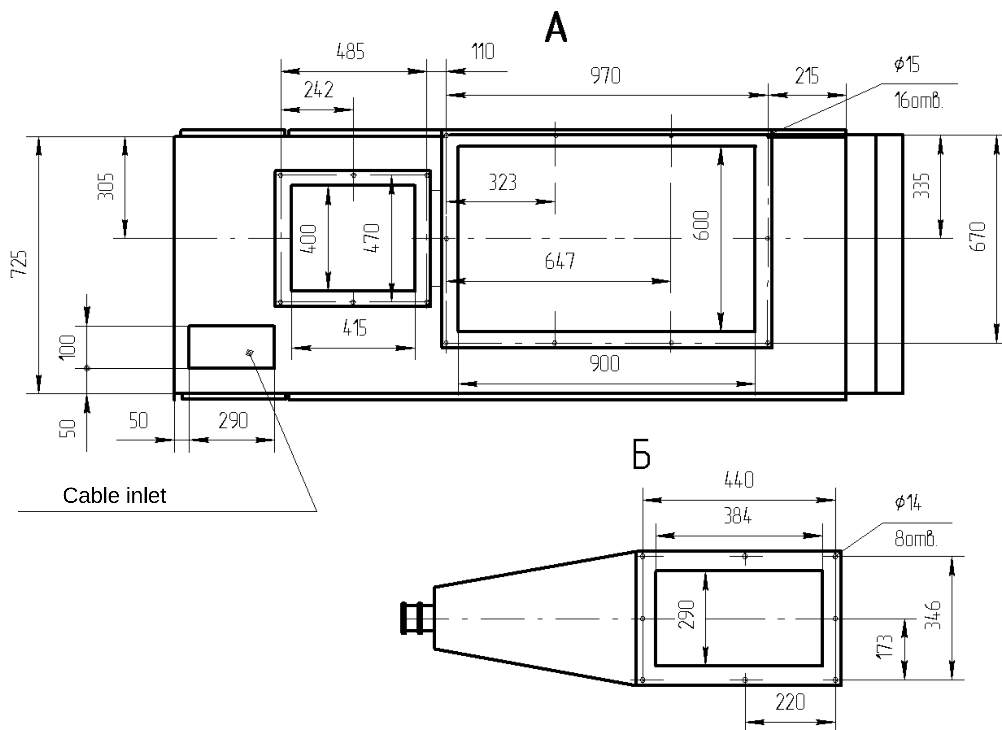
Sorting machine LS-20-05L
