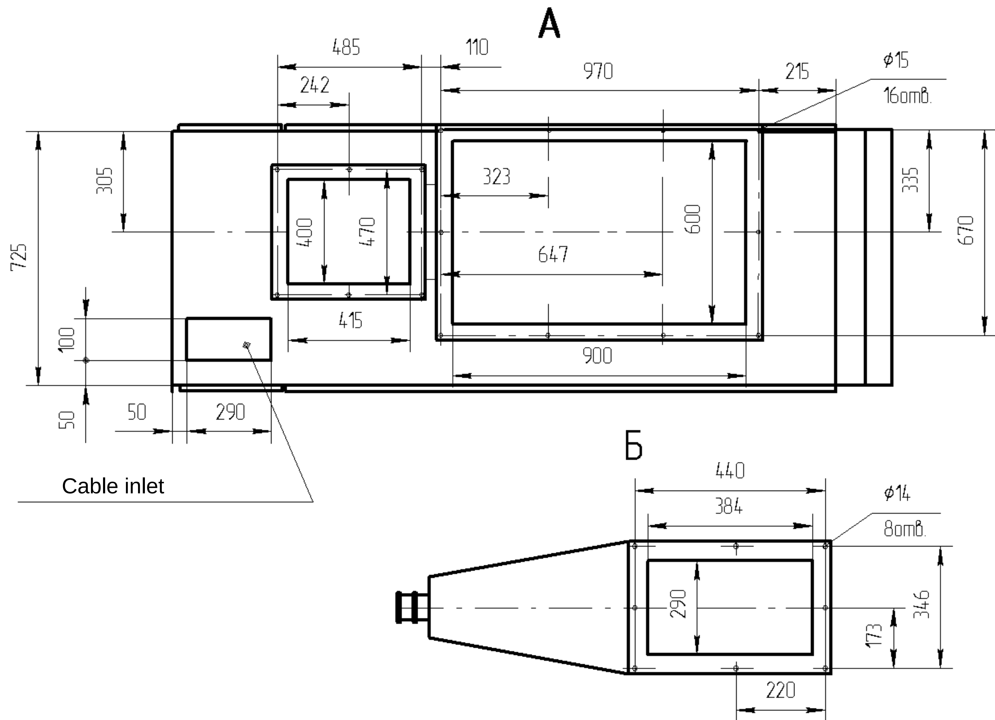
Sorting machine LS-20-05-2N
